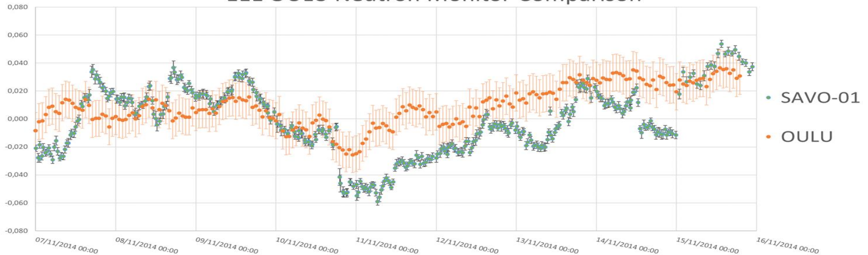
EEE OULU Neutron Monitor Comparison
